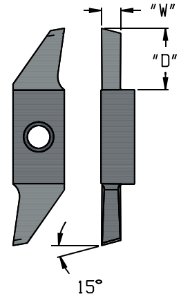
SWCR INSERTS
