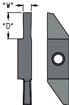
SWGL INSERTS
