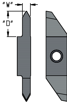
SWTL INSERTS
