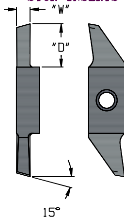
STCR INSERTS
