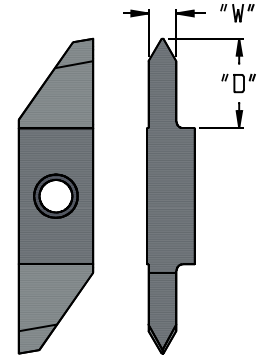
SWTR INSERTS
