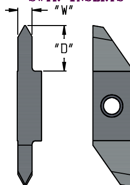
SWTR INSERTS
