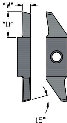
SWCL INSERTS
